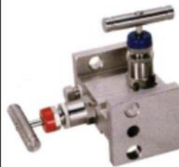
2 Valve Manifold Flange to Flange Type
